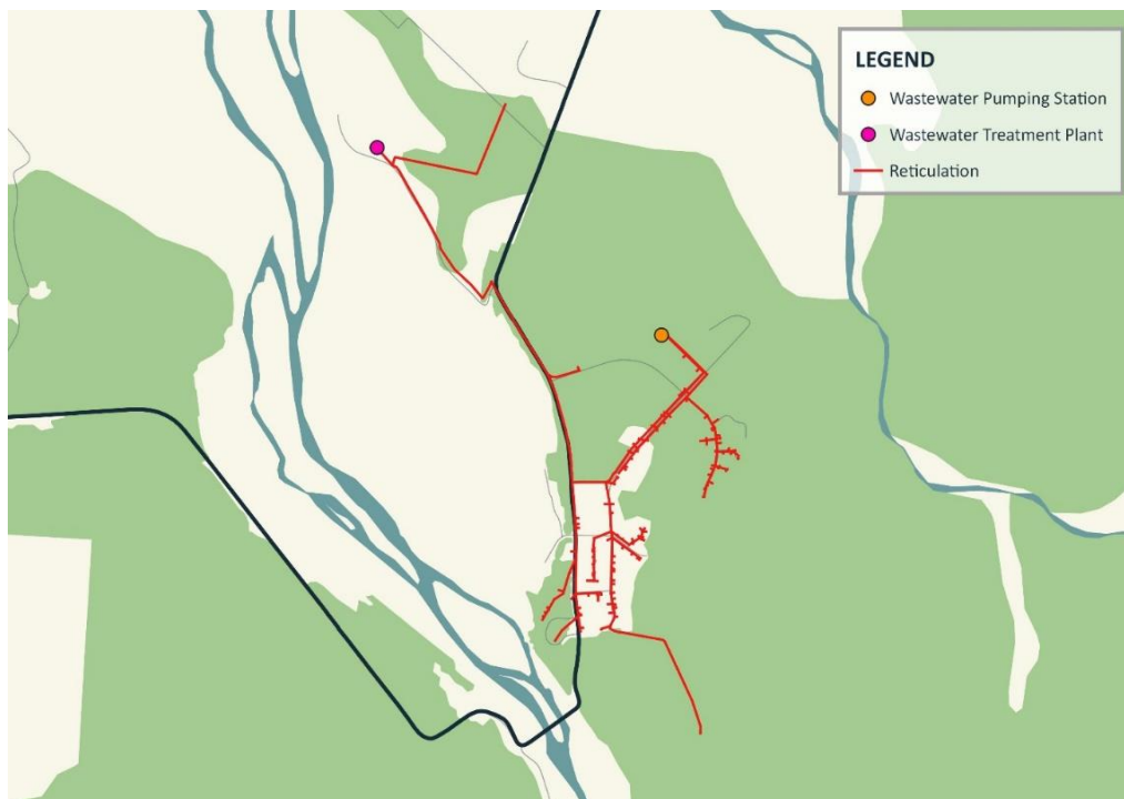
Figure 2-1: Franz Josef Scheme Map.
