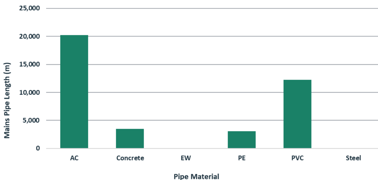
Figure 1-2: Hokitika Scheme Mains Pipe Material.
